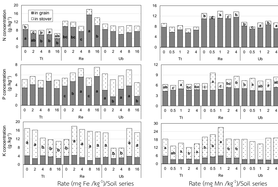
Different lowercase letters accompanying bars representing mean nutrient concentrations in grain or in stover within the same soil are significant different according to DMRT at p \leq 0.05
